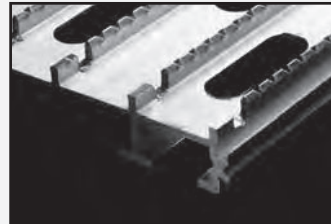
Non-Skid Ribs
